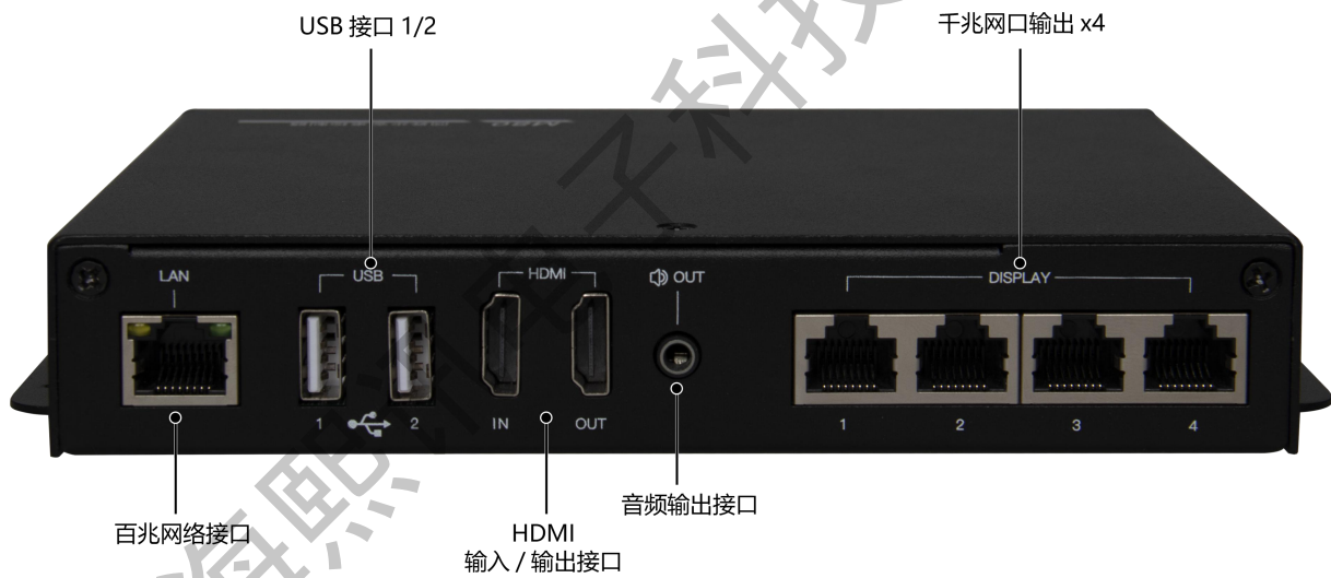
M80 后面板接口标注
