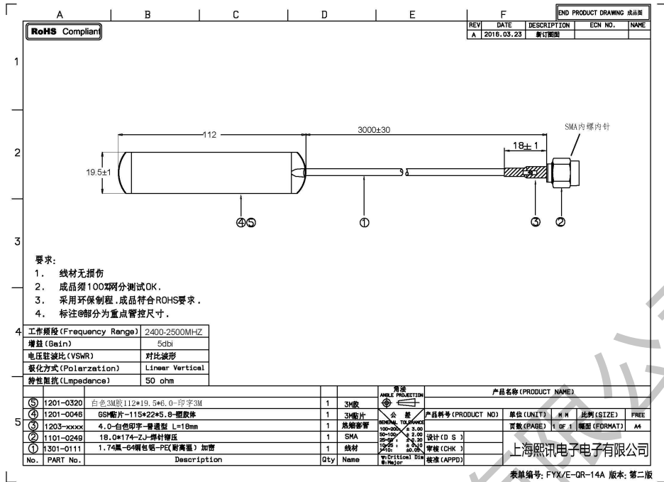
WiFi 贴片天线
